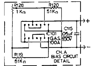
CH A BIAS CIRCUIT DETAIL
